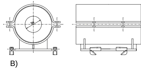
Fig. 9 : A) pre-insulated pipe support with clamping system RHS 1000 as guide support with lift-off lock (FLA) B) pre-insulated pipe support with clamping system RHS 4000 as guide support (FL)
