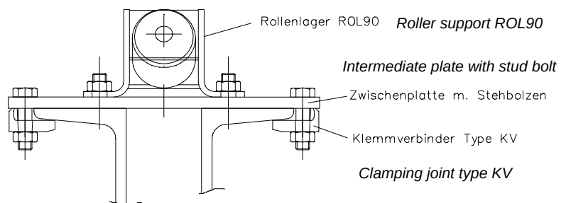
Figure 7 : roller support ROL90 with intermediate plate for double-U-profile
